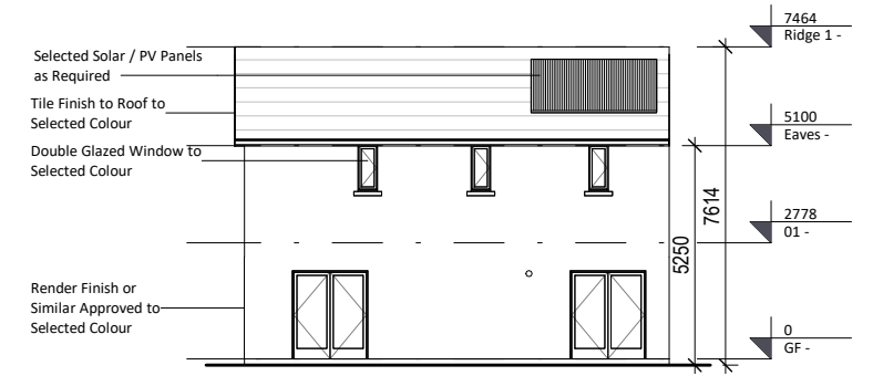
⑤ Rear Elevation Type A 1 : 200
