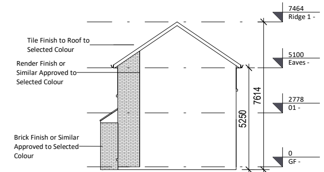
⑧ Gable End Elevation Type A (half brick) 1 : 200
