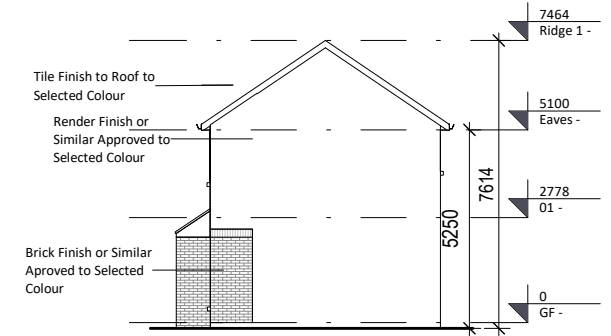
⑥ Gable End Elevation Type A (Half Brick) 1 : 200
