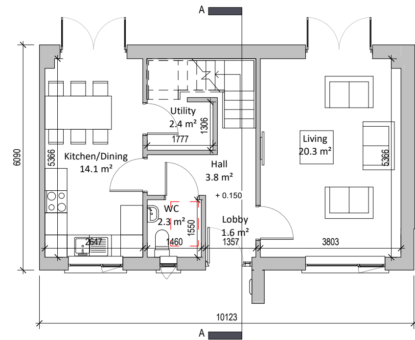
① Ground Floor Semi Detached 1 : 100
